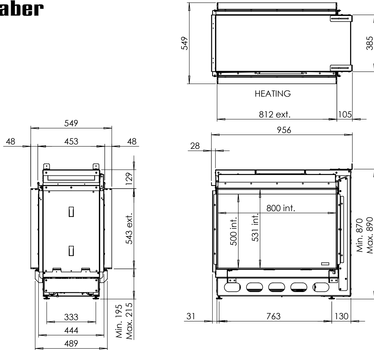
Dimensional Drawing e-Matrix Mood 800/500 ST
