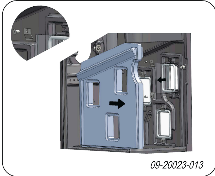
Side Heat Shield STEP 2, Only for SAGA107
