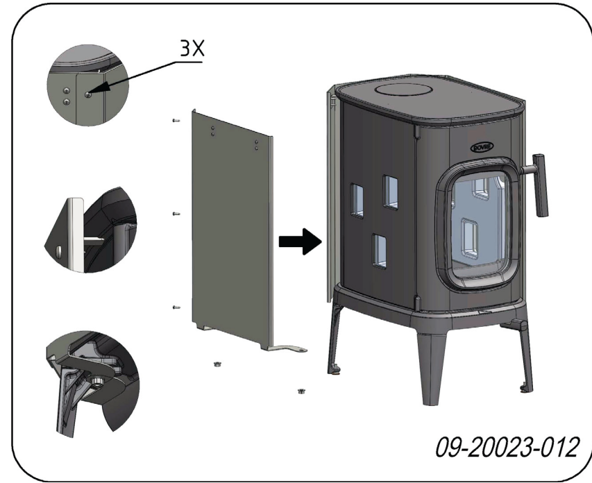
Side Heat Shield STEP 3, Only for SAGA 107
